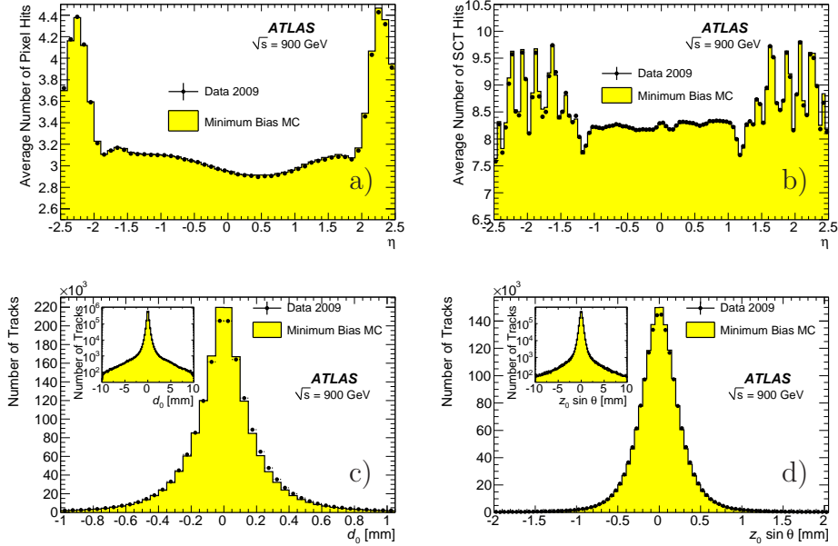
Figure 1: Comparison between data (dots) and minimum-bias ATLAS MC09 simulation (histograms) for the average number of Pixel hits (a) and SCT hits (b) per track as a function of \eta , and the transverse (c) and longitudinal (d) impact parameter distributions of the reconstructed tracks. The MC distributions in (c) and (d) are normalised to the number of tracks in the data. The inserts in the lower panels show the distributions in logarithmic scale.
